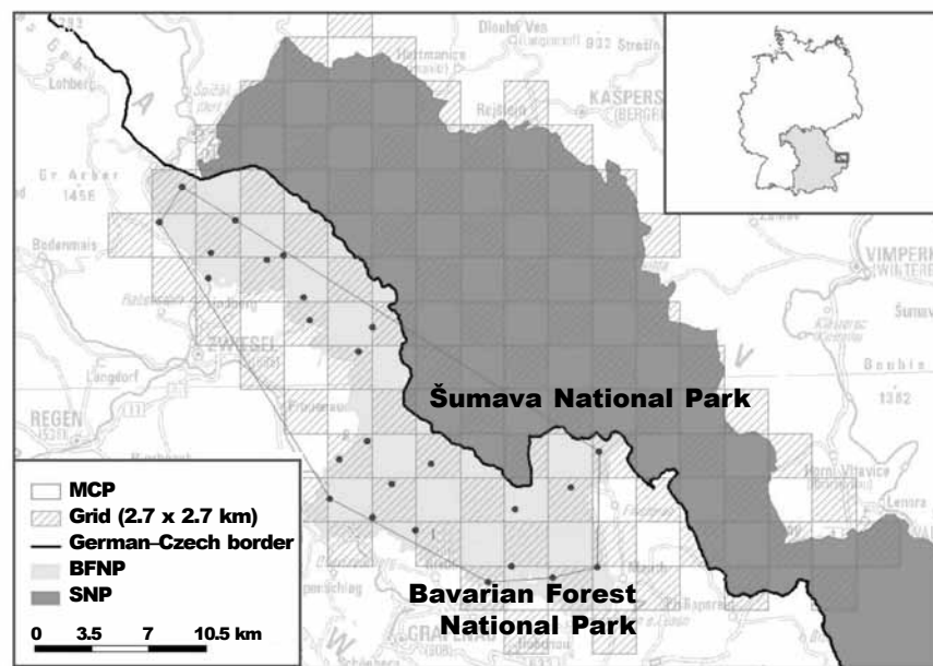
Fig. 1. Map of the Bavarian Forest National Park (BFNP) and Šumava National Park (SNP) showing the grid ( 2.7 \times 2.7 km) used to position the 24 camera trapping sites (•). The study area was defined as the minimum convex polygon (MCP) of the camera trapping sites.
