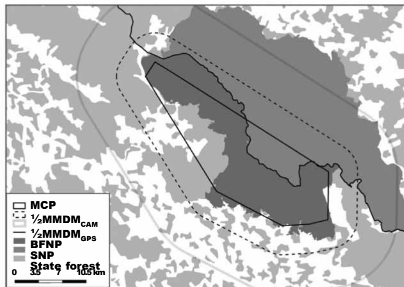
Fig. 3. Map showing the study area (black solid line) and two estimates for the effective study area obtained with a buffer radius of \frac{1}{2}MMDM_{CAM} (black dashed line) and \frac{1}{2}MMDM_{GPS} (grey solid line).
